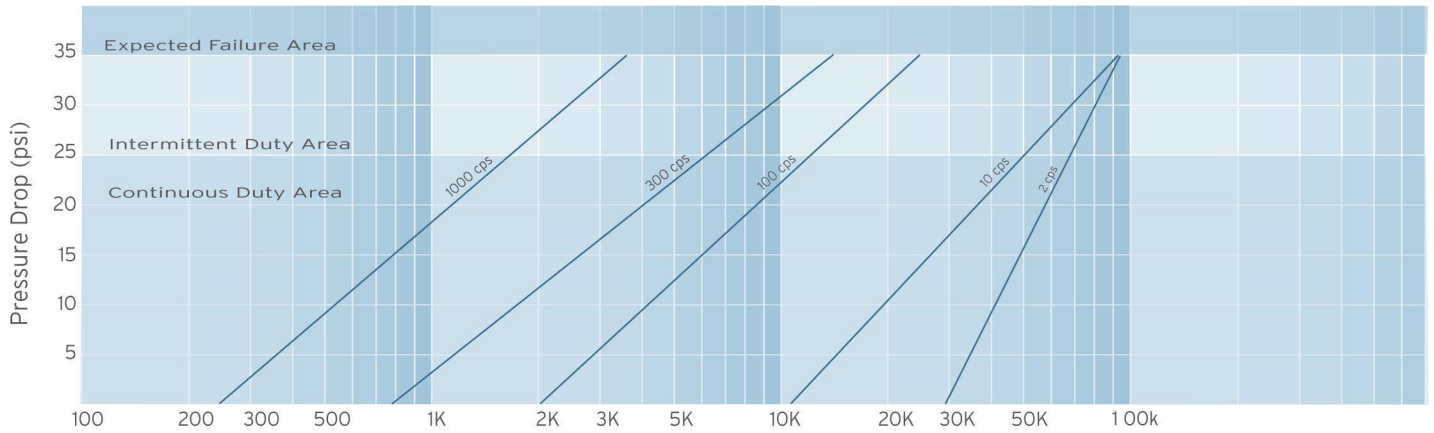
TYPICAL PRESSURE DROP (versus flow rate for various viscosities) (Using 10 Micron Element)
